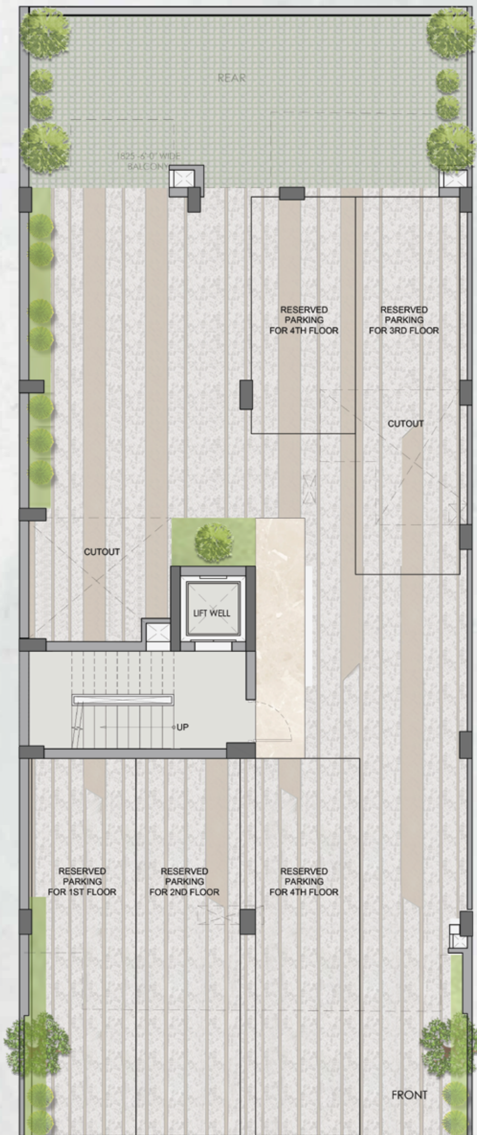
STILT FLOOR PLAN
