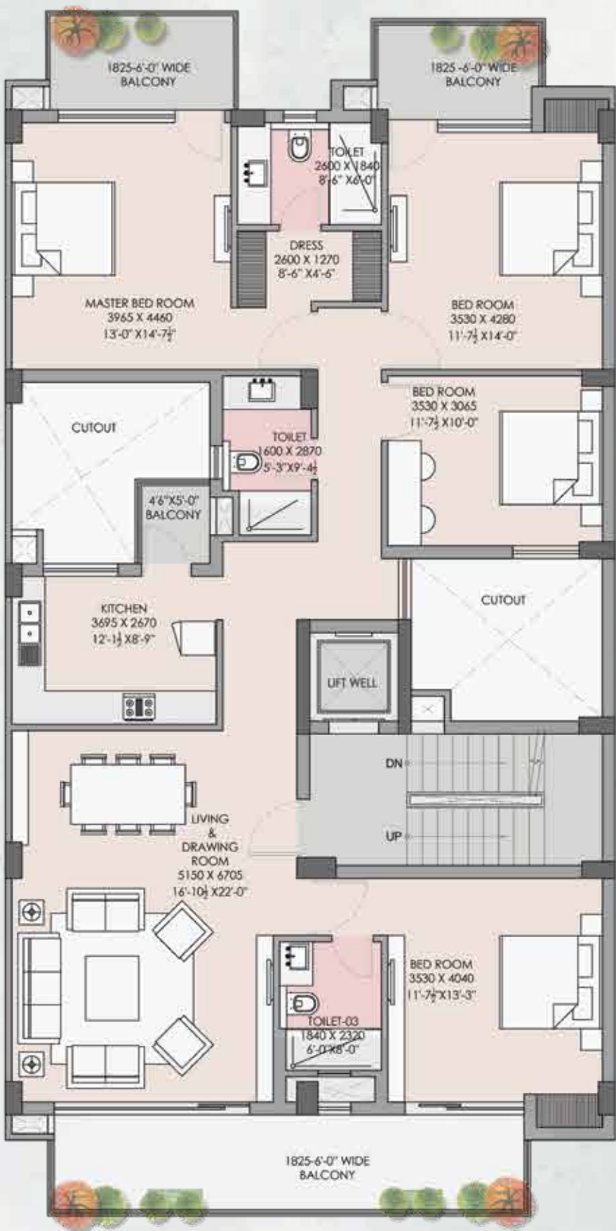
1st TO 4th TYPICAL FLOOR PLAN
