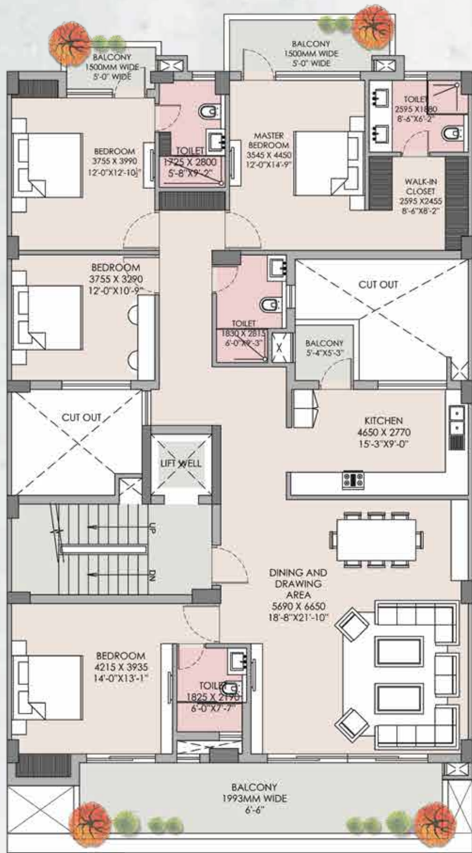
1st TO 4th TYPICAL FLOOR PLAN
